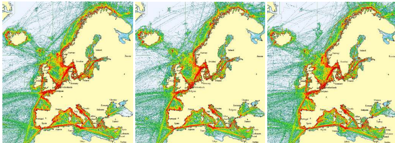
Figure 8: All ship types: ship traffic density in June 2019 (left), in June 2020 (centre) and in June 2021 (right)
