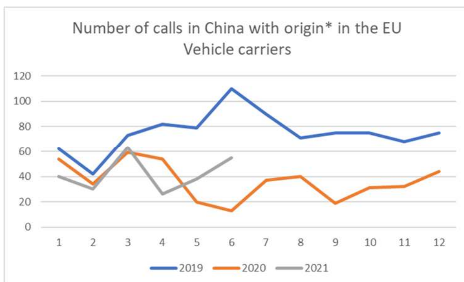
Figure 37: Total number of calls in China for vehicle carriers with origin in the EU in 2019, 2020 and 2021 (up to June 2021)
