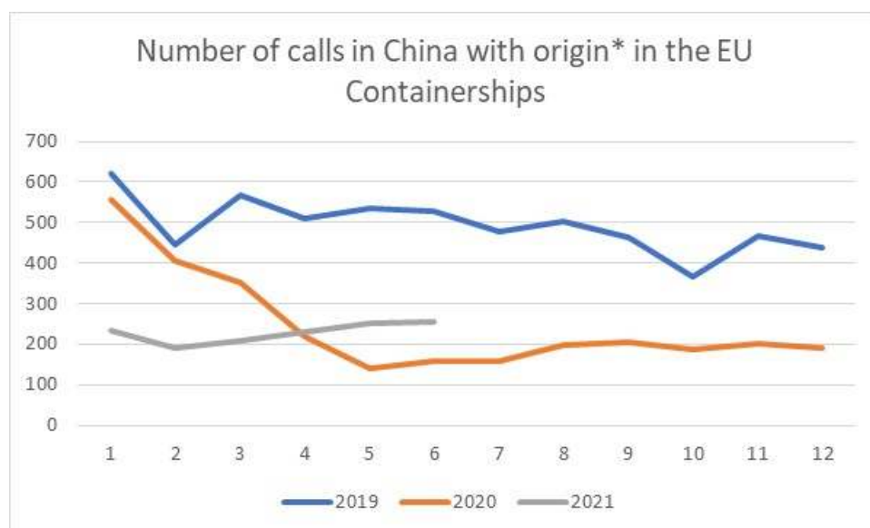
Figure 36: Total number of calls in China for container ships with origin in the EU in 2019, 2020 and 2021 (up to June 2021)
